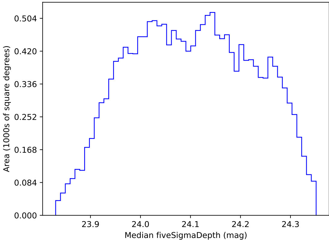
roll_pause_mjdp365_v3.4_10yrs WFD r band: Median fiveSigmaDepth
