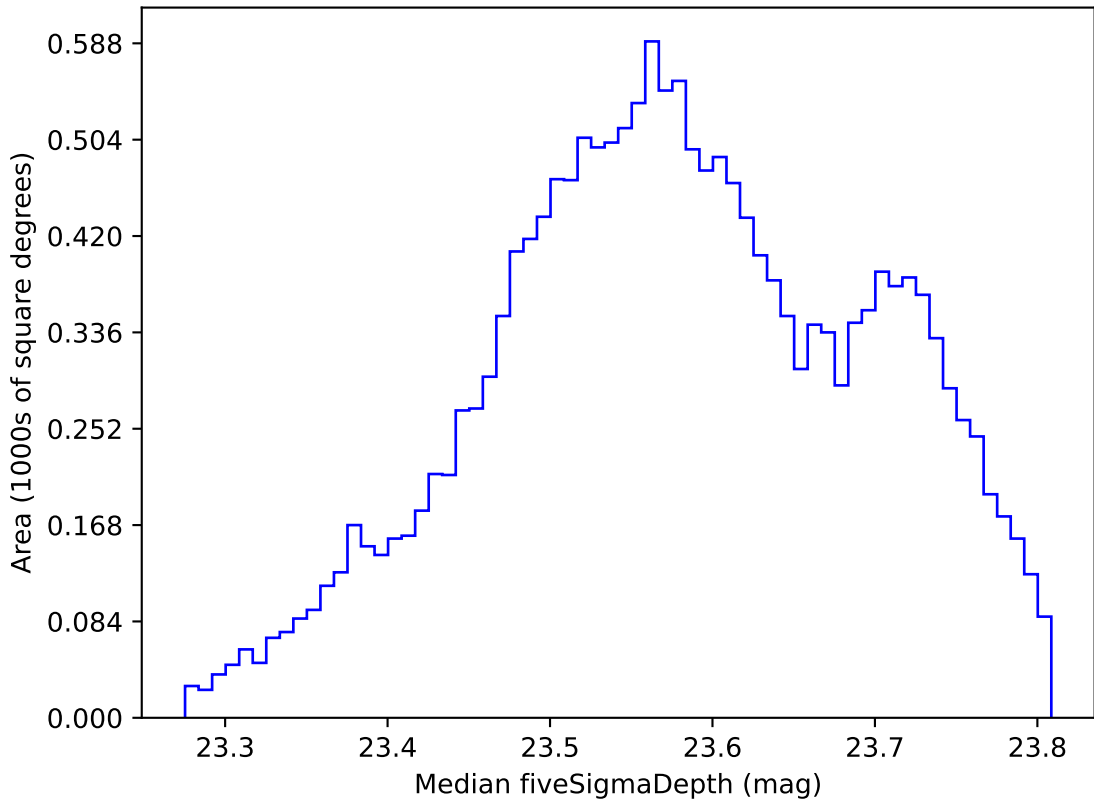
roll_pause_mjdp365_v3.4_10yrs WFD i band: Median fiveSigmaDepth
