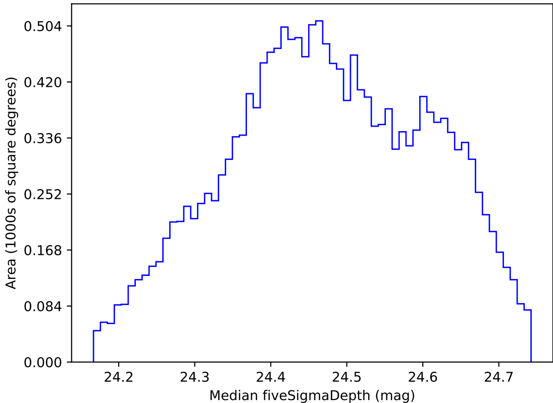
roll_pause_mjdp365_v3.4_10yrs WFD g band: Median fiveSigmaDepth
