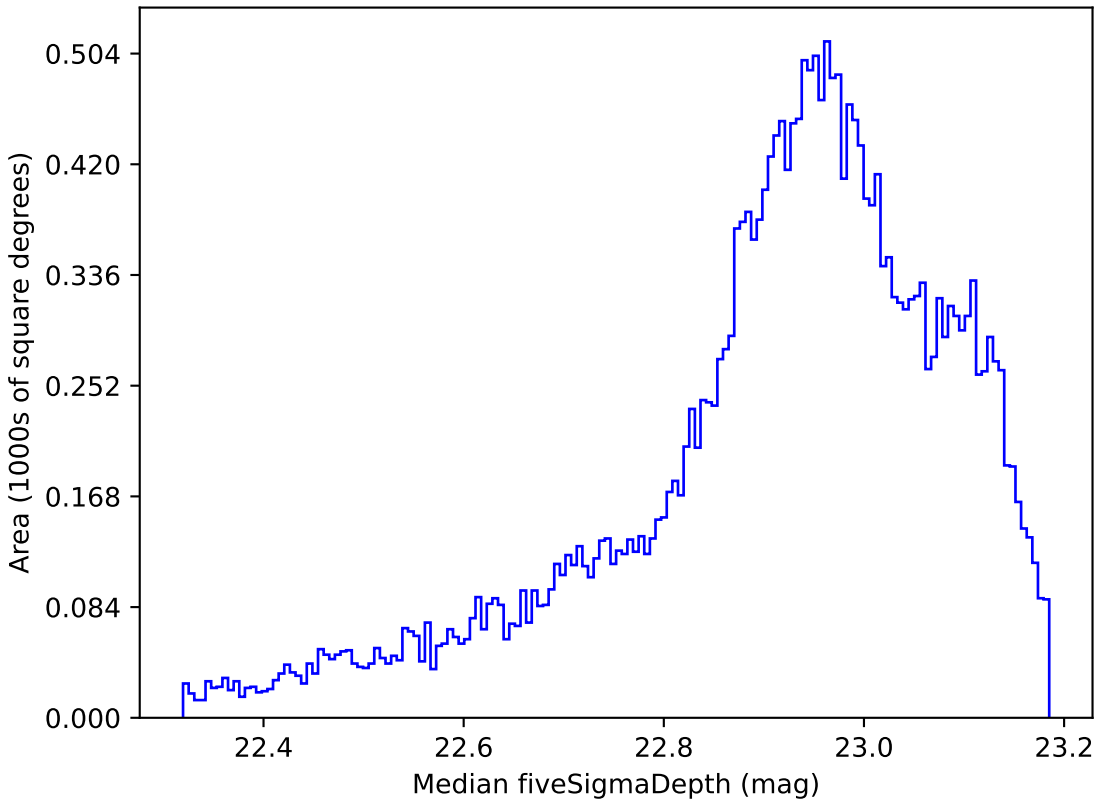
roll_pause_mjdp365_v3.4_10yrs All sky z band: Median fiveSigmaDepth
