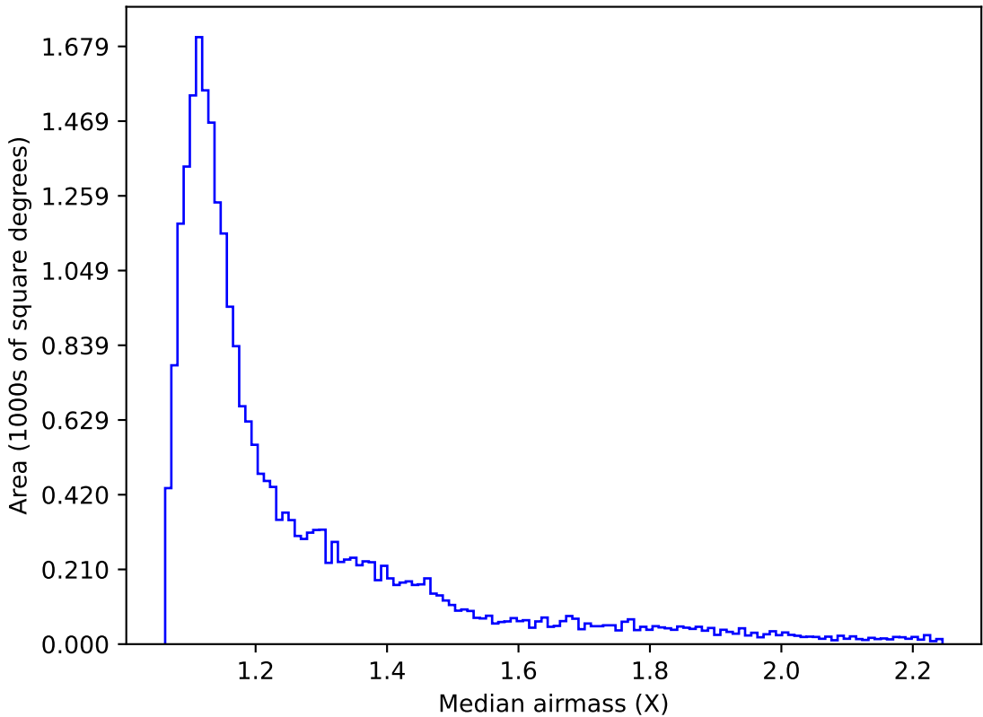
roll_pause_mjdp365_v3.4_10yrs Yr 1 z band: Median airmass
