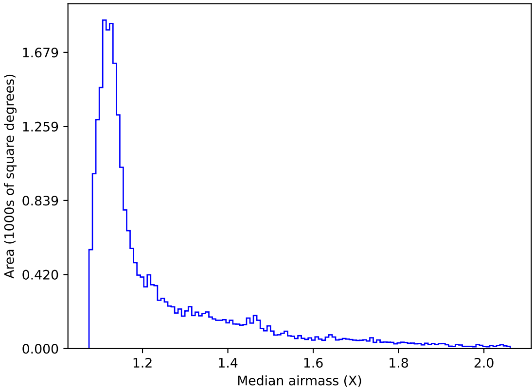
roll_pause_mjdp365_v3.4_10yrs Yr 1 all bands: Median airmass
