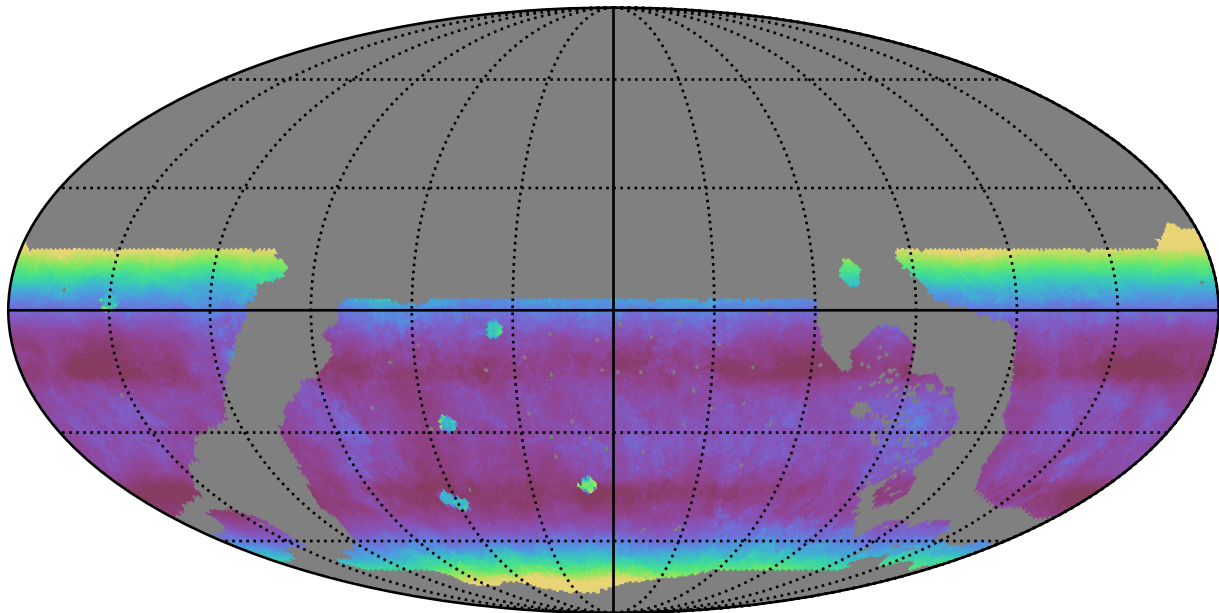
roll_pause_mjdp365_v3.4_10yrs WFD z band: Median airmass
