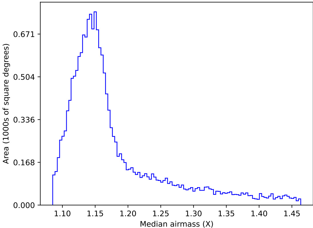
roll_pause_mjdp365_v3.4_10yrs WFD z band: Median airmass
