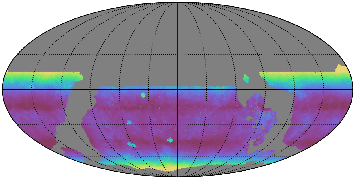
roll_pause_mjdp365_v3.4_10yrs WFD y band: Median airmass
