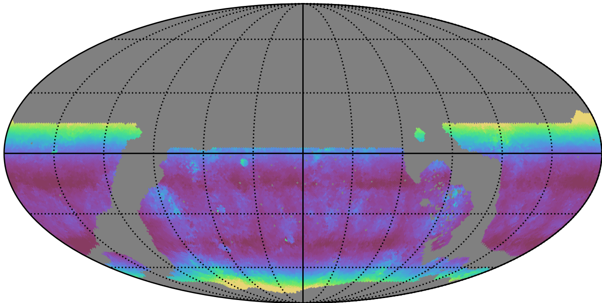
roll_pause_mjdp365_v3.4_10yrs WFD u band: Median airmass
