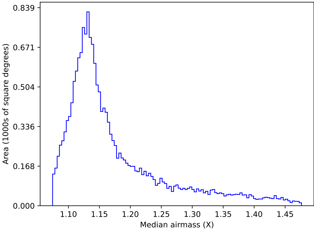
roll_pause_mjdp365_v3.4_10yrs WFD u band: Median airmass
