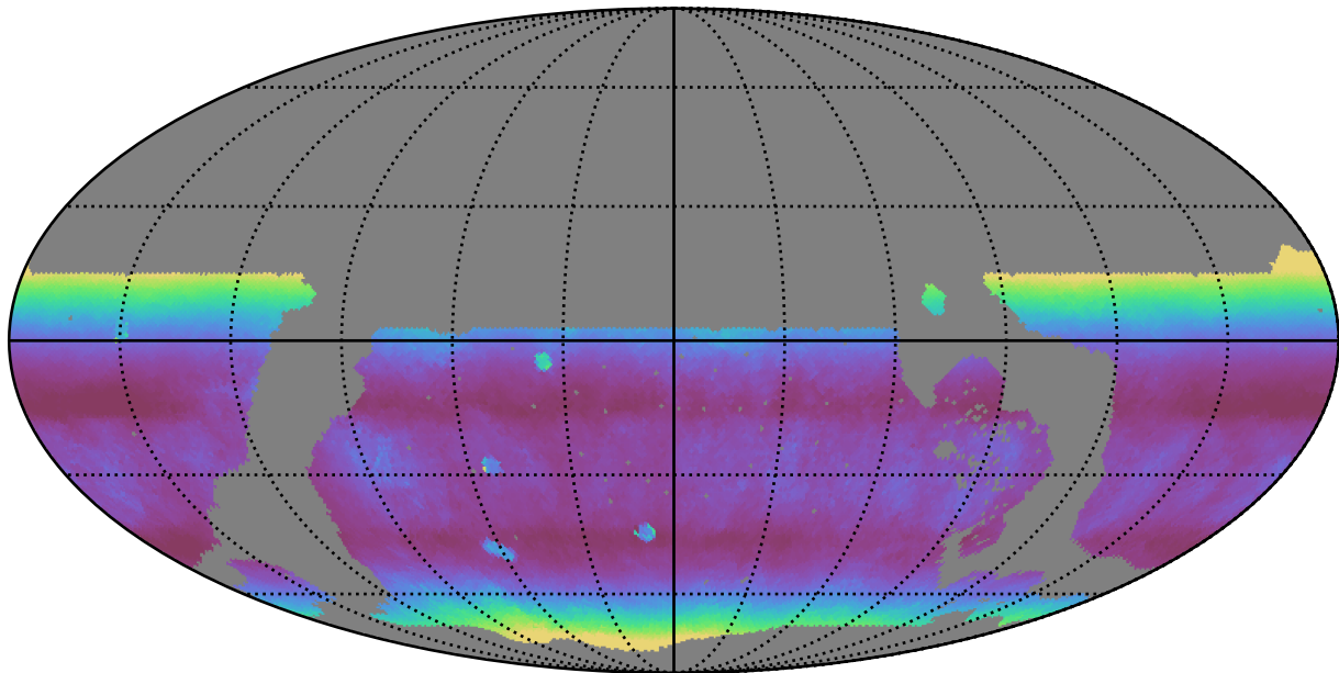
roll_pause_mjdp365_v3.4_10yrs WFD r band: Median airmass
