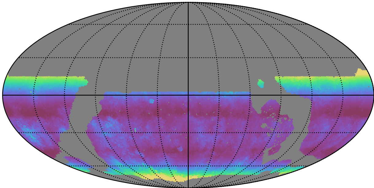
roll_pause_mjdp365_v3.4_10yrs WFD g band: Median airmass
