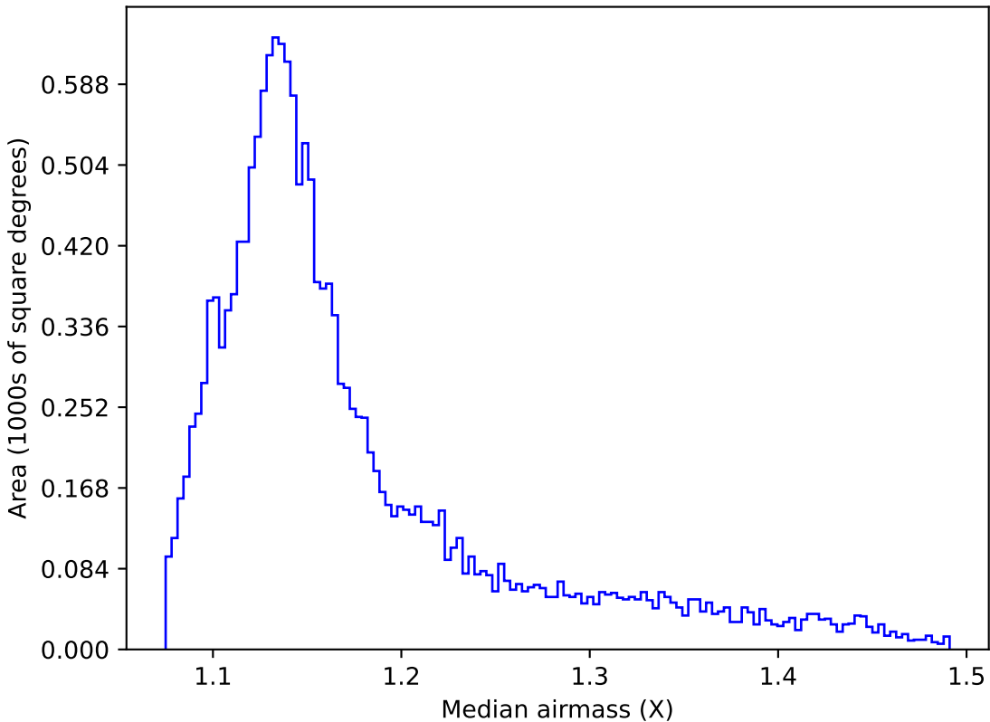
roll_pause_mjdp365_v3.4_10yrs WFD g band: Median airmass
