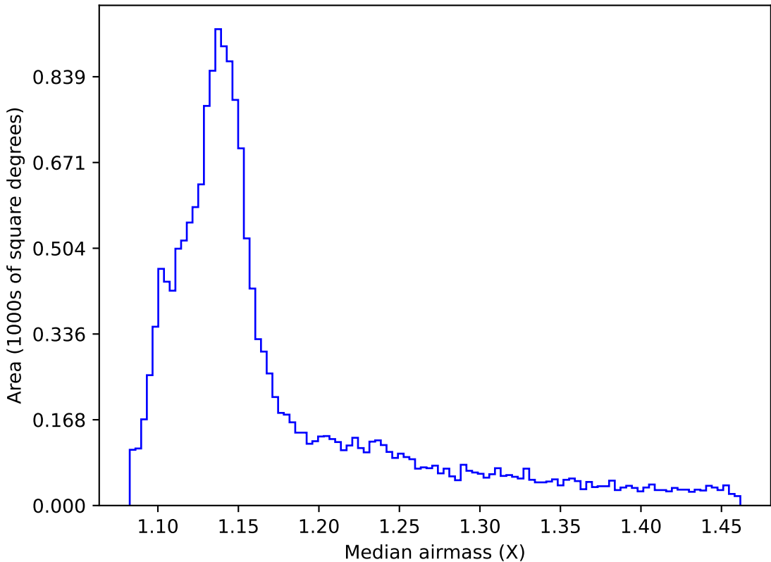
roll_pause_mjdp365_v3.4_10yrs WFD all bands: Median airmass
