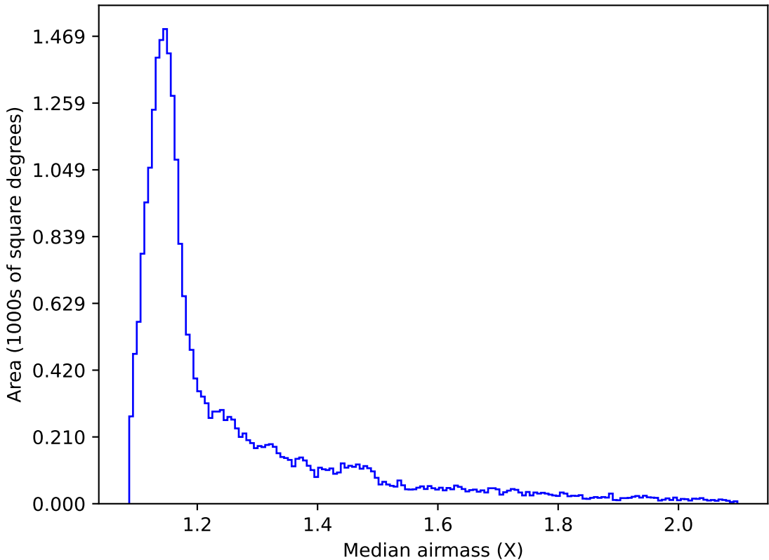
roll_pause_mjdp365_v3.4_10yrs All sky z band: Median airmass
