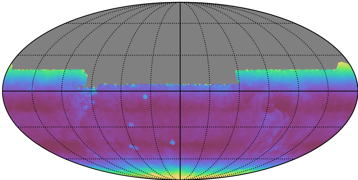
roll_pause_mjdp365_v3.4_10yrs All sky y band: Median airmass
