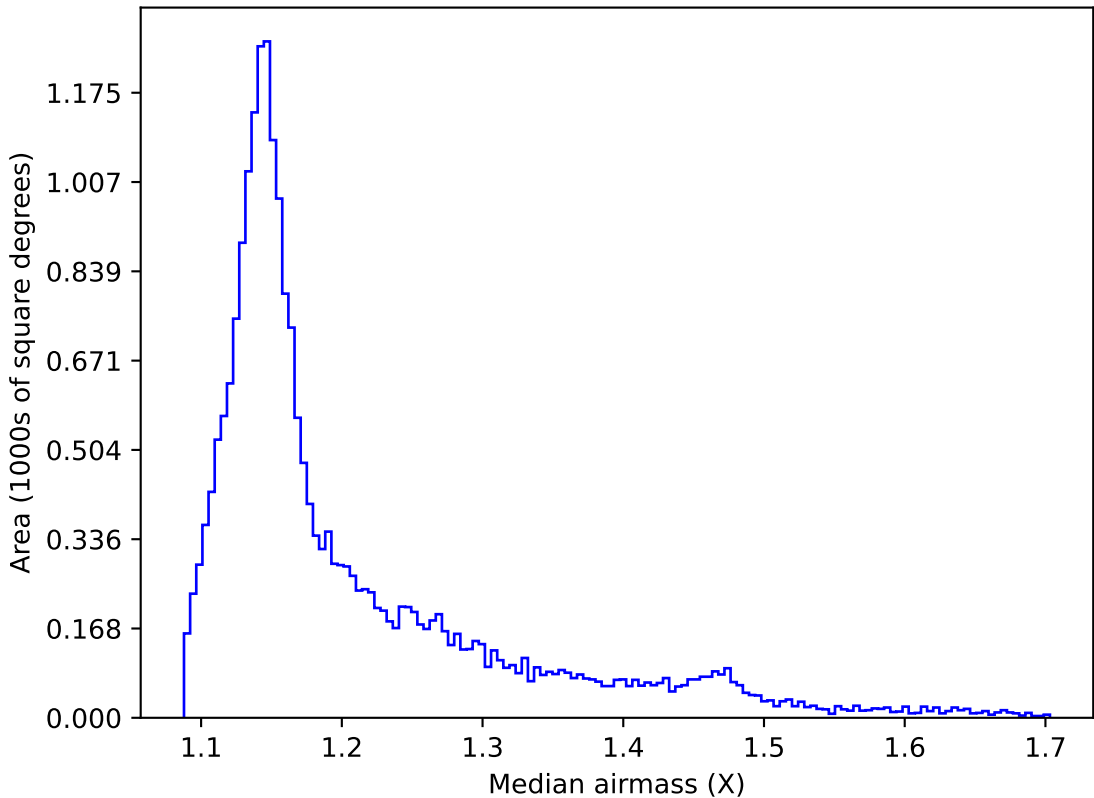
roll_pause_mjdp365_v3.4_10yrs All sky y band: Median airmass
