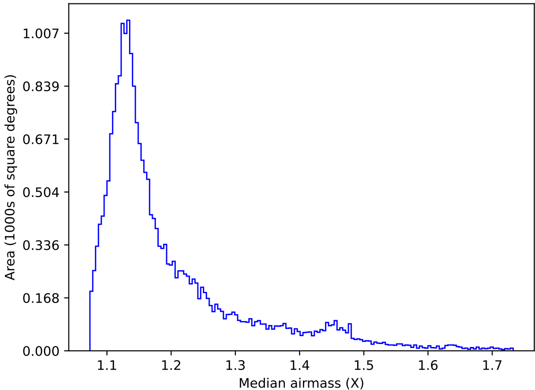
roll_pause_mjdp365_v3.4_10yrs All sky u band: Median airmass
