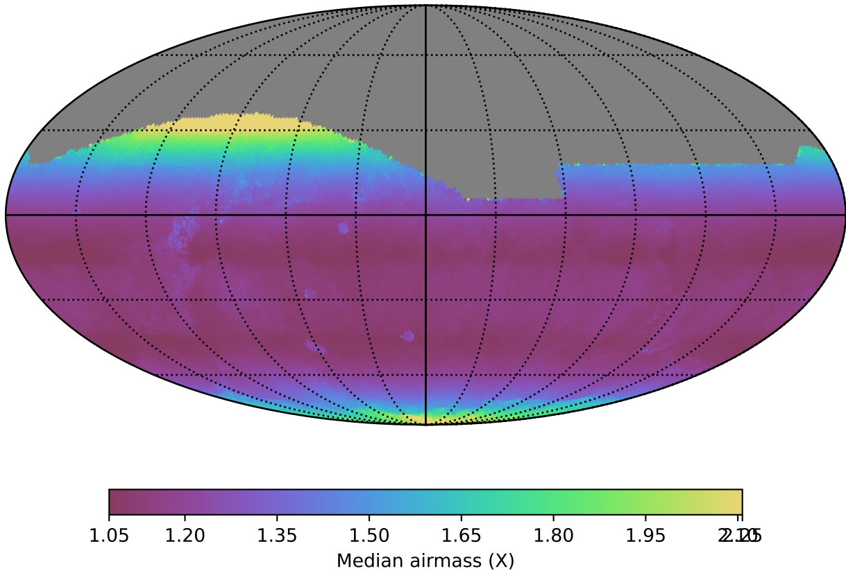
roll_pause_mjdp365_v3.4_10yrs All sky r band: Median airmass
