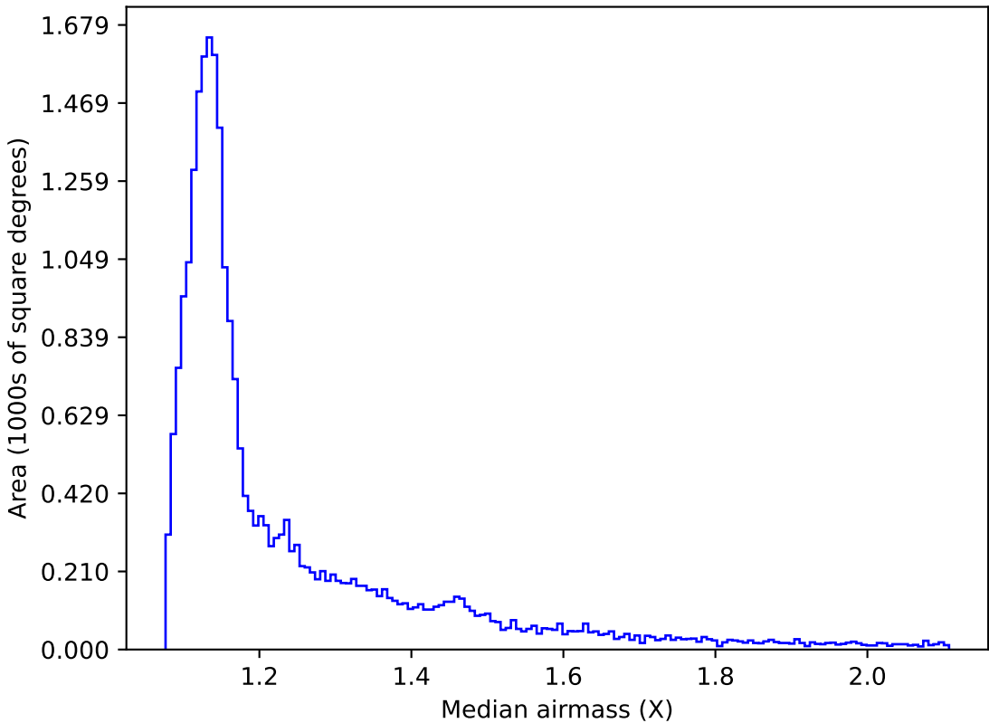
roll_pause_mjdp365_v3.4_10yrs All sky r band: Median airmass
