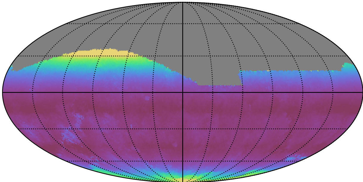
roll_pause_mjdp365_v3.4_10yrs All sky g band: Median airmass
