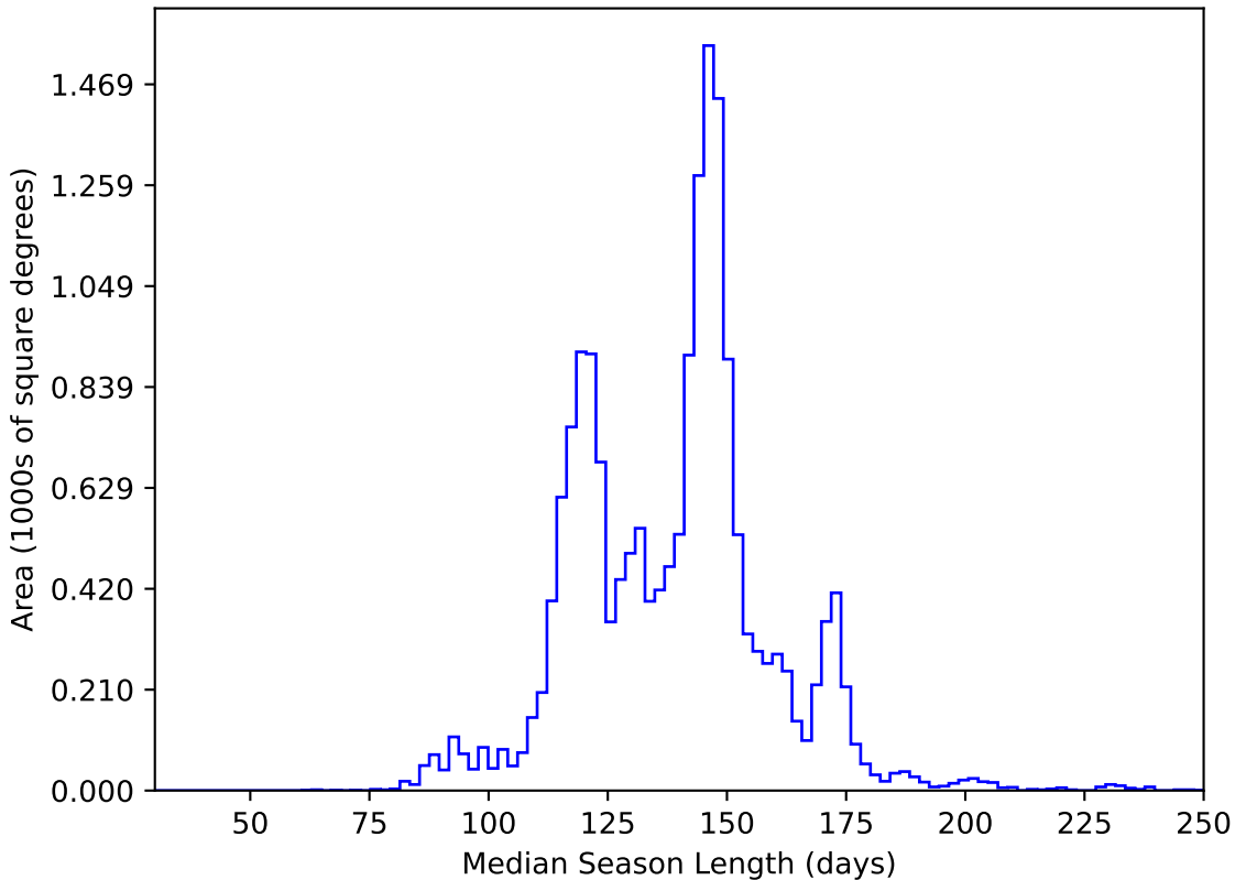
roll_pause_mjdp365_v3.4_10yrs WFD y band: Median Season Length
