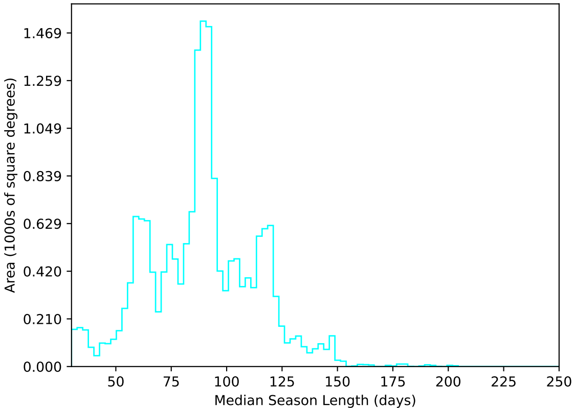
roll_pause_mjdp365_v3.4_10yrs WFD u band: Median Season Length
