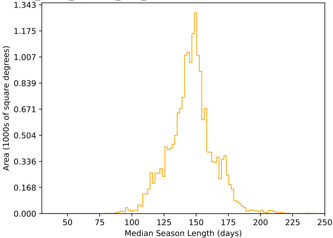
roll_pause_mjdp365_v3.4_10yrs WFD r band: Median Season Length
