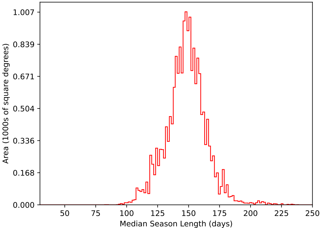
roll_pause_mjdp365_v3.4_10yrs WFD i band: Median Season Length
