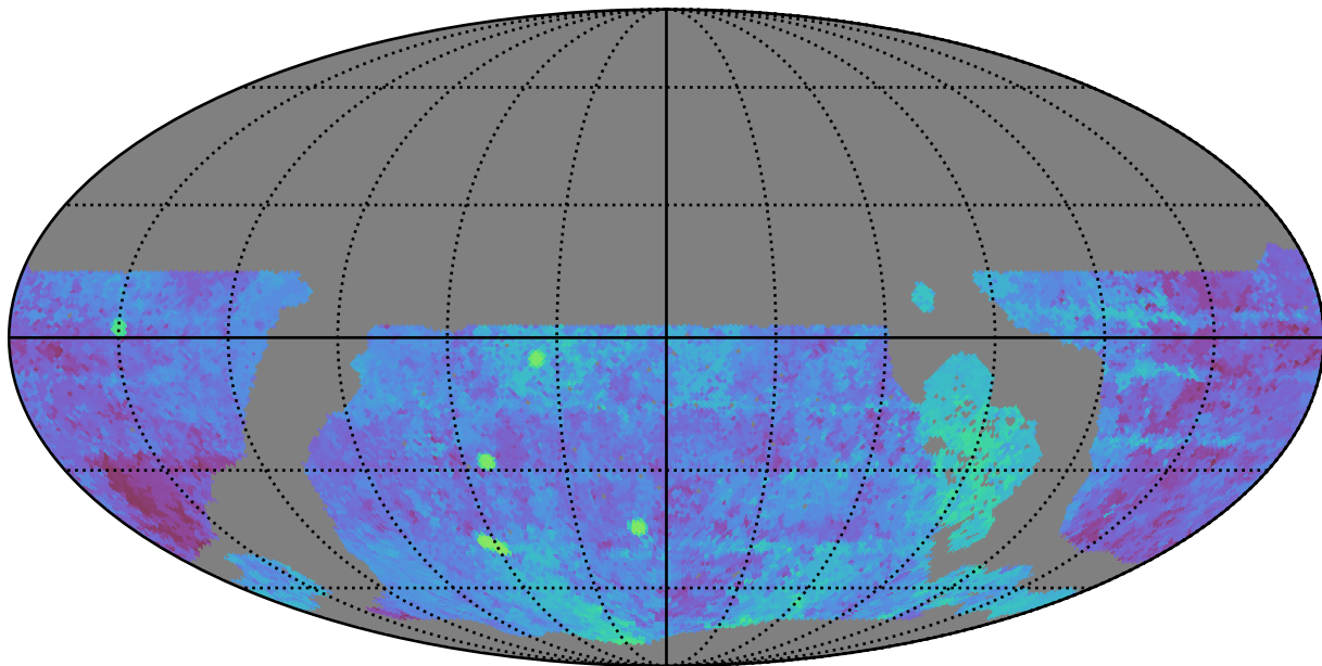
roll_pause_mjdp365_v3.4_10yrs WFD g band: Median Season Length
