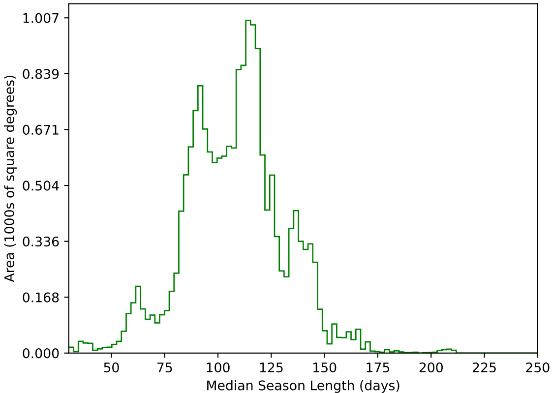
roll_pause_mjdp365_v3.4_10yrs WFD g band: Median Season Length
