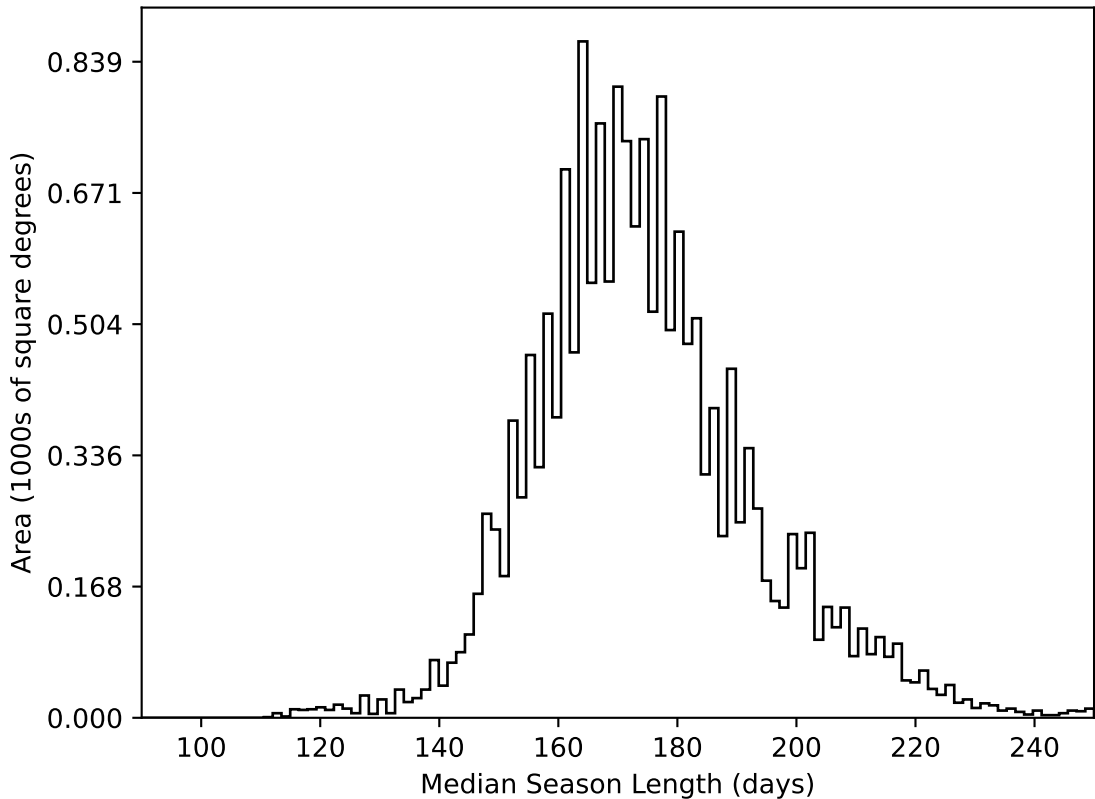
roll_pause_mjdp365_v3.4_10yrs WFD all bands: Median Season Length
