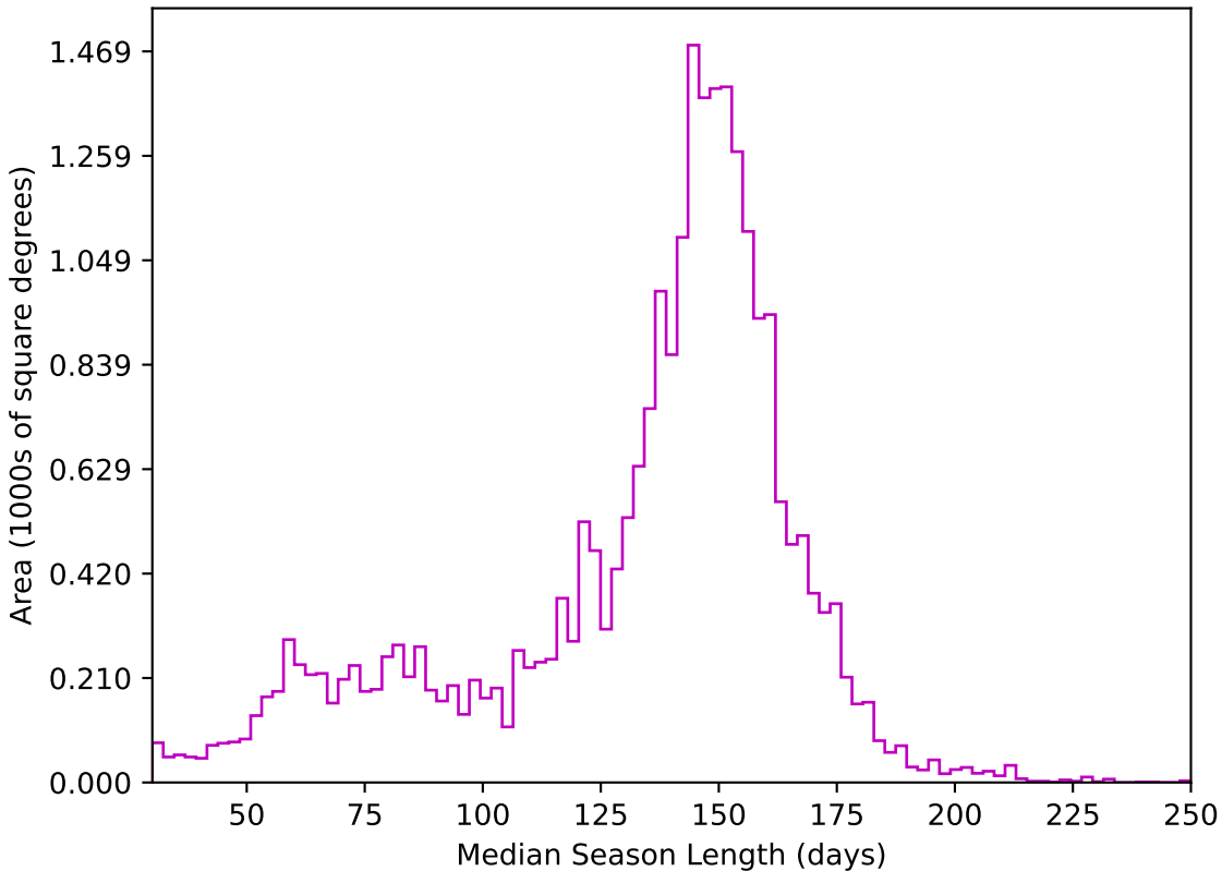
roll_pause_mjdp365_v3.4_10yrs All sky z band: Median Season Length
