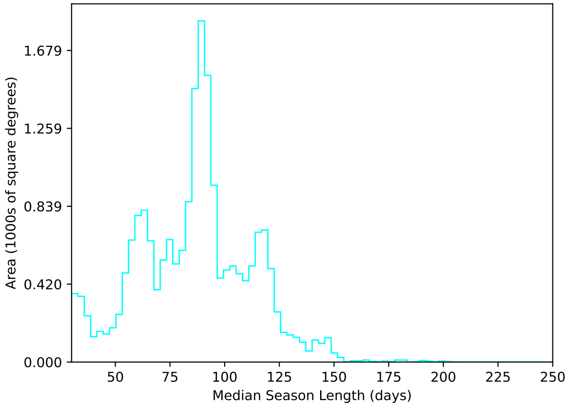
roll_pause_mjdp365_v3.4_10yrs All sky u band: Median Season Length
