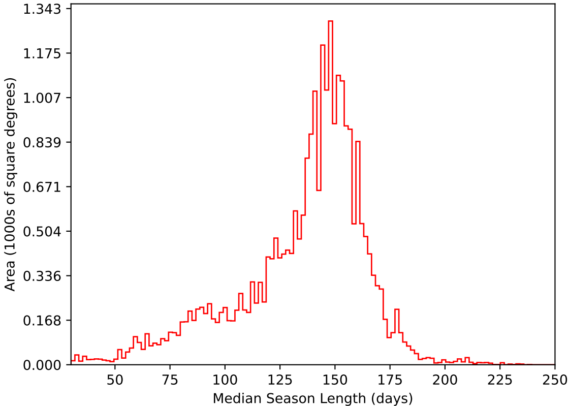
roll_pause_mjdp365_v3.4_10yrs All sky i band: Median Season Length
