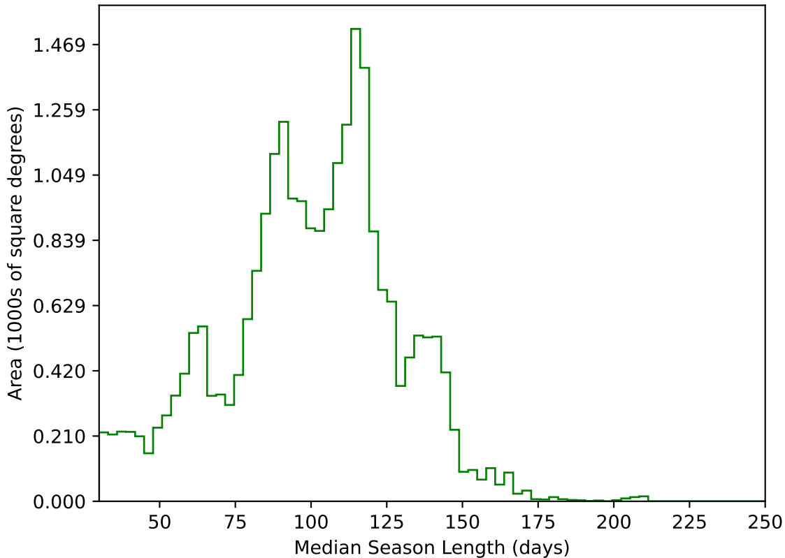
roll_pause_mjdp365_v3.4_10yrs All sky g band: Median Season Length
