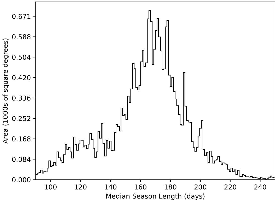
roll_pause_mjdp365_v3.4_10yrs All sky all bands: Median Season Length
