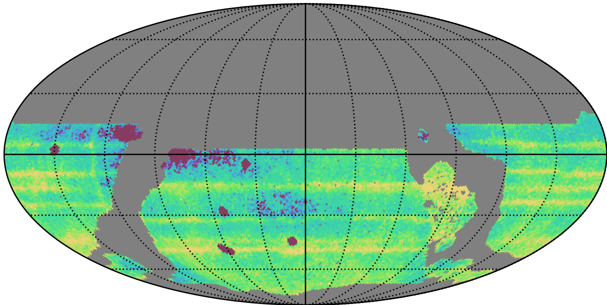
roll_pause_mjdp365_v3.4_10yrs WFD: Median Intra-Night Gap
