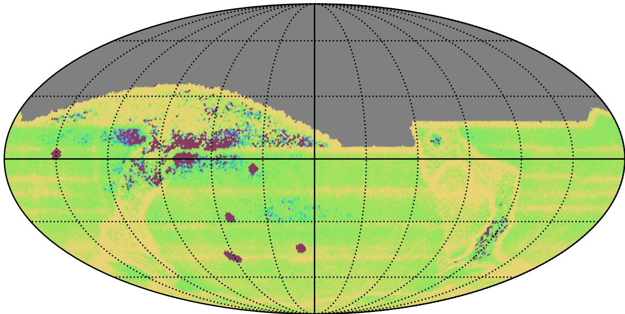
roll_pause_mjdp365_v3.4_10yrs All sky: Median Intra-Night Gap
