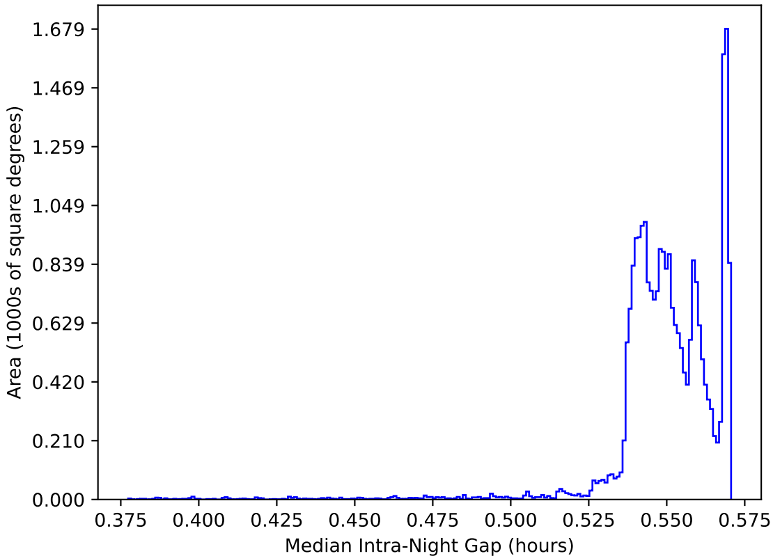
roll_pause_mjdp365_v3.4_10yrs All sky: Median Intra-Night Gap
