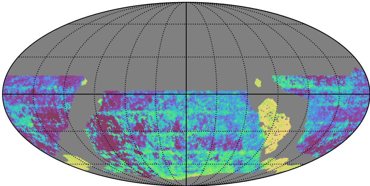
roll_pause_mjdp365_v3.4_10yrs WFD y band: Median Inter-Night Gap
