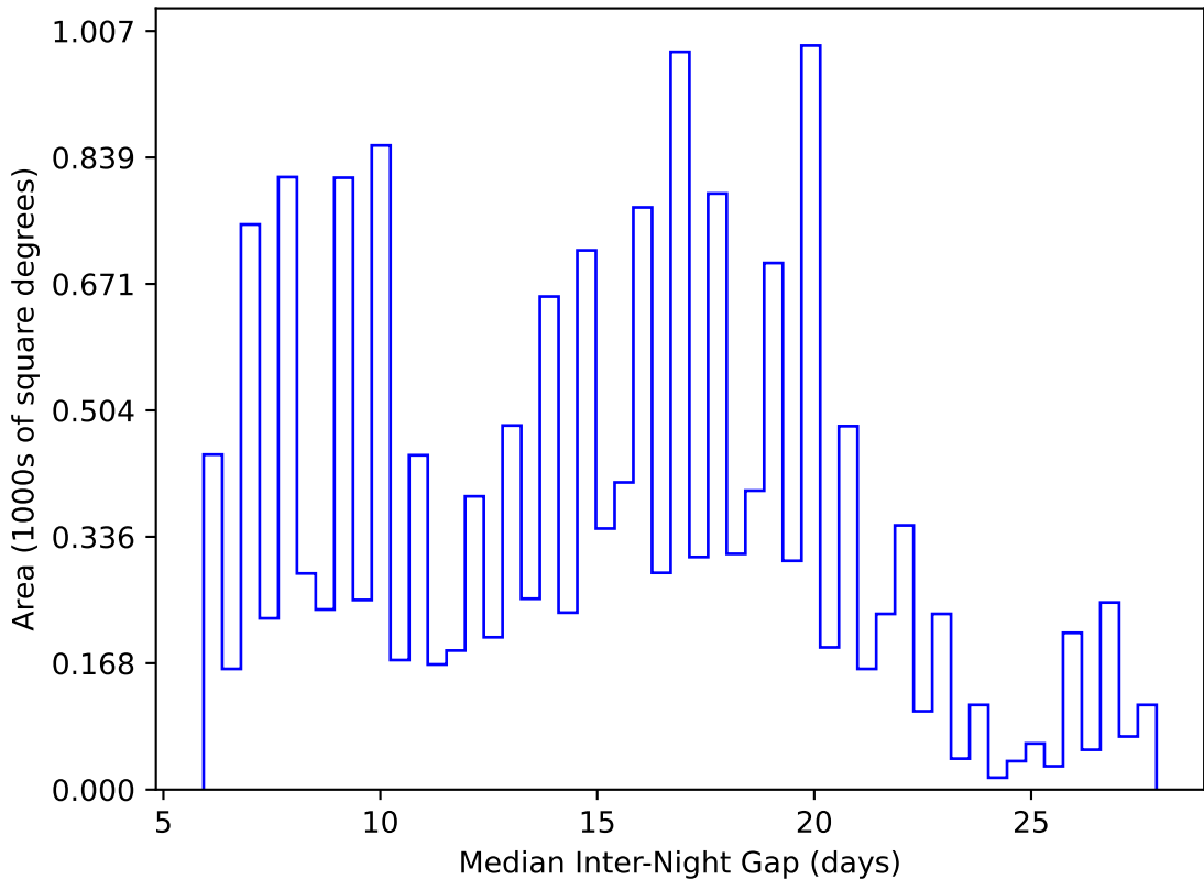
roll_pause_mjdp365_v3.4_10yrs WFD y band: Median Inter-Night Gap
