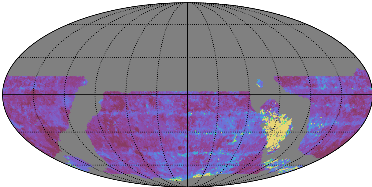
roll_pause_mjdp365_v3.4_10yrs WFD u band: Median Inter-Night Gap
