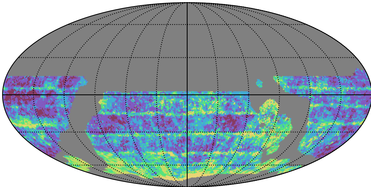
roll_pause_mjdp365_v3.4_10yrs WFD r band: Median Inter-Night Gap
