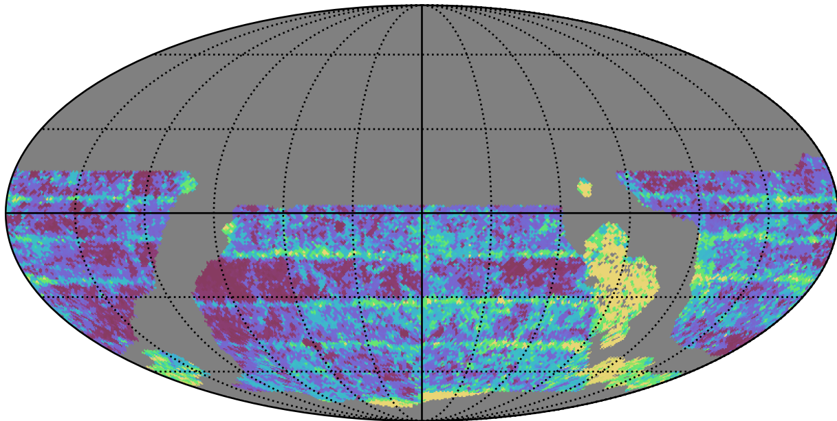
roll_pause_mjdp365_v3.4_10yrs WFD i band: Median Inter-Night Gap
