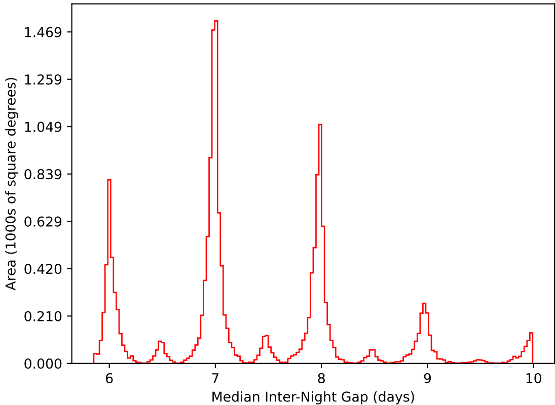
roll_pause_mjdp365_v3.4_10yrs WFD i band: Median Inter-Night Gap
