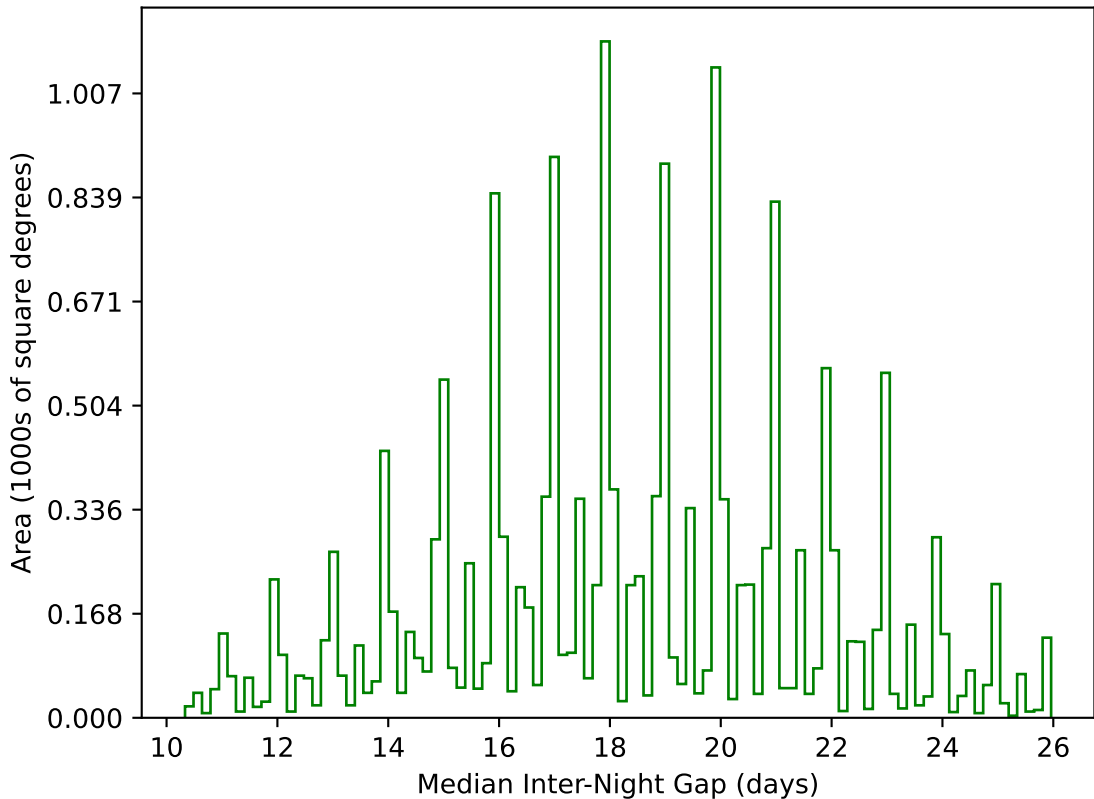
roll_pause_mjdp365_v3.4_10yrs WFD g band: Median Inter-Night Gap
