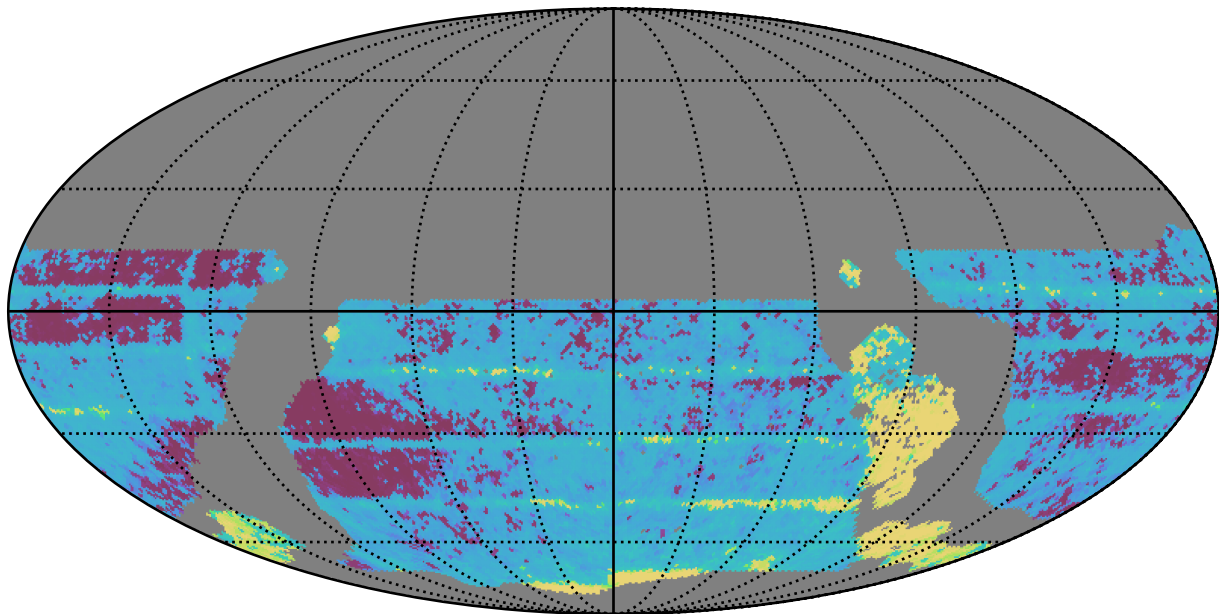
roll_pause_mjdp365_v3.4_10yrs WFD all bands: Median Inter-Night Gap
