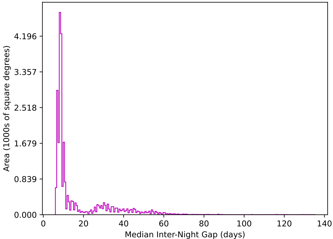
roll_pause_mjdp365_v3.4_10yrs All sky z band: Median Inter-Night Gap
