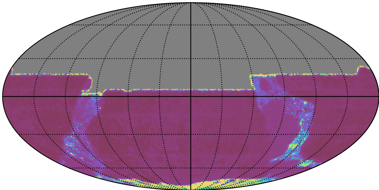
roll_pause_mjdp365_v3.4_10yrs All sky y band: Median Inter-Night Gap
