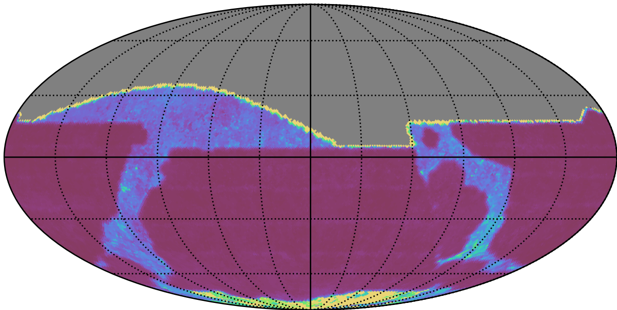
roll_pause_mjdp365_v3.4_10yrs All sky r band: Median Inter-Night Gap
