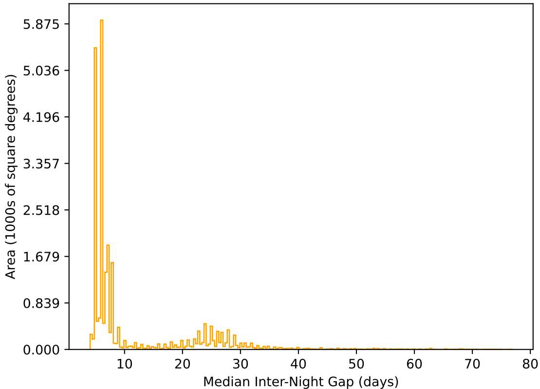
roll_pause_mjdp365_v3.4_10yrs All sky r band: Median Inter-Night Gap
