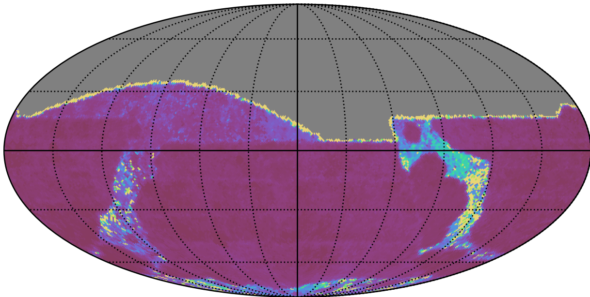
roll_pause_mjdp365_v3.4_10yrs All sky g band: Median Inter-Night Gap
